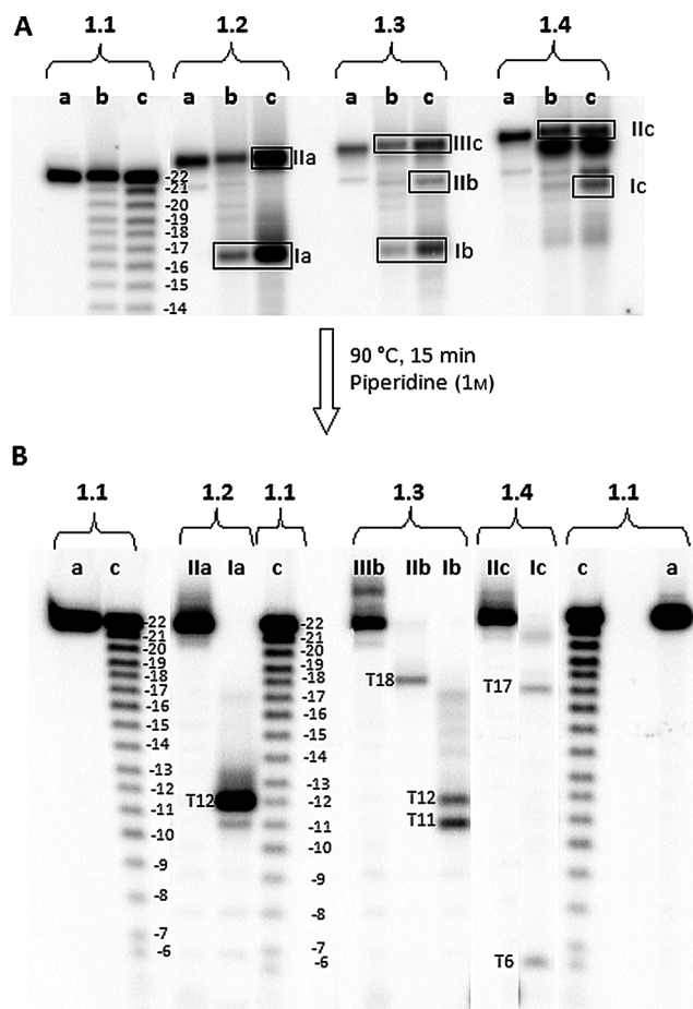
Figure 3. Denaturing gel electrophoresis of alkylated products of 22AG in K^+ -rich buffer. A) 3'-Exonuclease digestion of bands 1.1–1.4 obtained by alkylation with PDC-PEG-Bp (see Figure 1A): enzyme units/ \mu L: lane a, 0; lane b, 0.04; lane c, 0.08. Band 1.1 corresponds to non-alkylated 22AG. B) Treatment of the digested fragments with piperidine. The numbered pyrimidine sites correspond to the digestion arrests.
