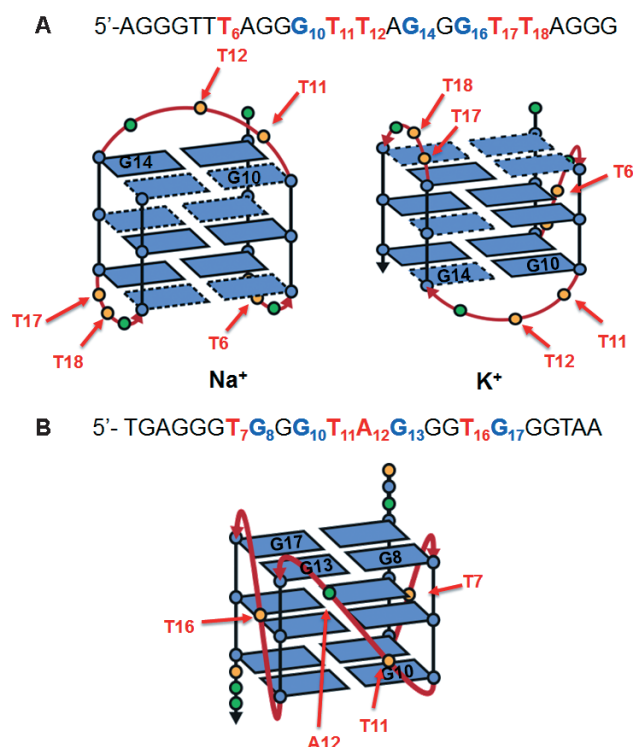
Figure 5. A) Schematic structure of the human telomeric G4 in Na^+ - and in K^+ -rich buffer, and sites alkylated by PDC-Bp and PDC-N 3 derivatives. B) Schematic structure of the c-myc 22G4T-G23T G4 and sites alkylated by PDC-N 3 derivatives. Guanine residues are represented by blue squares (G-quartets, dashed squares are syn and plain squares are anti ) or blue spheres (G-loops); yellow and green spheres stand for T and A in the loops, respectively. Alkylated guanine residues are labeled in black; alkylated nucleobases in the loops are shown with red arrows.
