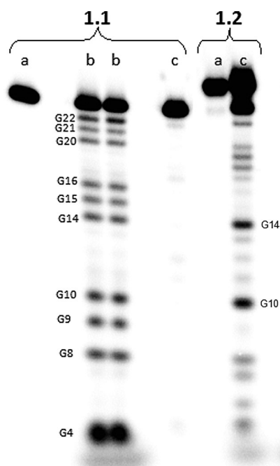
Figure 4. Denaturing gel electrophoresis of alkylated products of 22AG in K^+ -rich buffer. Treatment with piperidine of bands 1.1 and 1.2 obtained by alkylation with PDC-PEG-N 3 (see Figure 1 B): lane a: non-treated sample; lane b: sample (band 1.1, which corresponds to non-alkylated 22AG) treated with DMS (dimethyl sulfate) and piperidine to give a reference scale for fragment migration; lane c: piperidine-treated sample.
