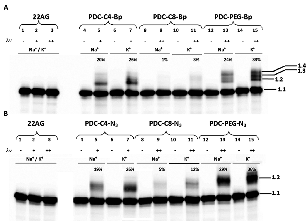
Figure 1. Denaturing gel electrophoresis (15% acrylamide) of the alkylation products of 22AG (10 μM) in the presence of Na + and K + buffer (100 mM) with A) PDC-C4-Bp , PDC-C8-Bp , and PDC-PEG-Bp , and B) PDC-C4-N 3 , PDC-C8-N 3 , and PDC-PEG-N 3 (25 μM). Lanes 1, 2, 3, 4, 6, 8, 10, 12, and 14 are control experiments that show the effect of no irradiation (lane 1, 4, 6, 8, 10, 12, and 14) and irradiation for 90 flashes (lane 2) and 150 flashes (lane 3). Lanes 5 and 7 show the results of irradiation at 360 nm for 90 flashes; lanes 9, 11, 13, and 15 show the results of irradiation at 360 nm for 150 flashes. Bands have been numbered with respect to their migration as compared to a control (band 1.1: no migration; bands 1.2, 1.3, 1.4: retarded bands, numbered in the order of the extent of migration). λν: – absence of irradiation, + 90 flashes, ++ 150 flashes.
