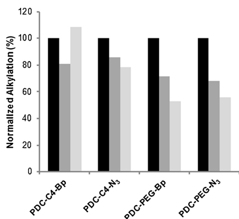
Figure 2. Quantitative analysis of the alkylation of the telomeric sequence 22AG (10 \mu M, 100 mM K^+ -rich buffer) by the PDC-XL derivatives (25 \mu M) in the absence (black bars) or in the presence of a competitor (80 \mu M): ds lac (dark-gray bars), 22A g mut (light-gray bars).
