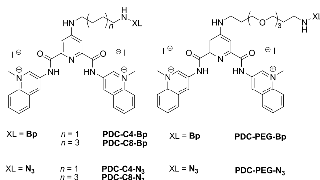
Scheme 1. Detailed chemical structure of the six PDC-XL derivatives synthesized in this study.
